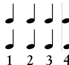
Figure 3. Transcription of phasing broken-rhythm (attack above, defence below)
